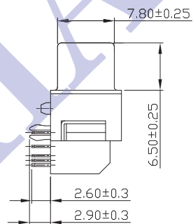
D7210 (鉚合無螺絲)
